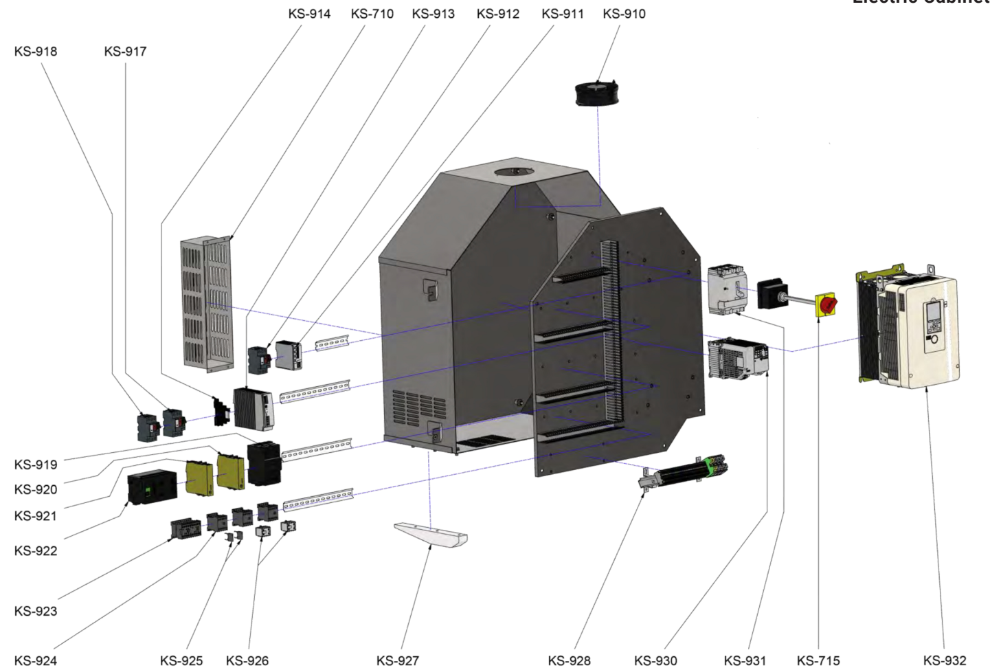
Electric Cabinet
